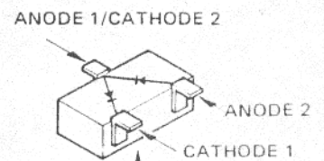
Marked Surface 1SS226(C3) (D2013)
