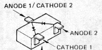
Marked Surface 1SS226(C3) (D1015)
