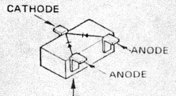
Marked Surface 1SS184(B3) (D2010,2011,2012)
