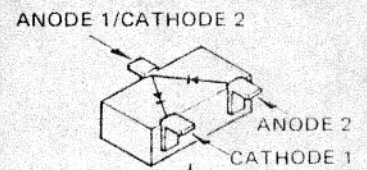
Marked Surface 1SS226(C3) (D2013)
