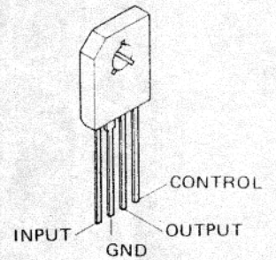
LA5005H (Q1004)
