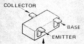
Marked Surface 2SA812(M6/M7) (Q2015,2017,2020) 2SA1162GR(SG) (Q2019,2021) 2SC1623(L6/L7) (Q2001,2003,2016, 2018,2022) 2SC2620B(QB) (Q2005,2010) 2SC2759(U22) (Q2011,2012) 2SC3120(HB) (Q2009)
