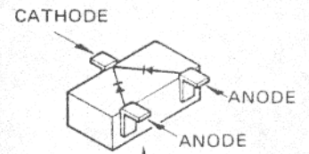
Marked Surface 1SS184(B3) (D2010,2011,2012)
